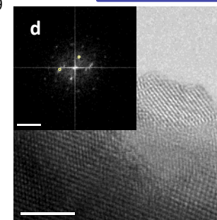
HRTEM image of a-ZITO film grown at 400 °C, showing a crystalline ZITO phase embedded in a disordered matrix
