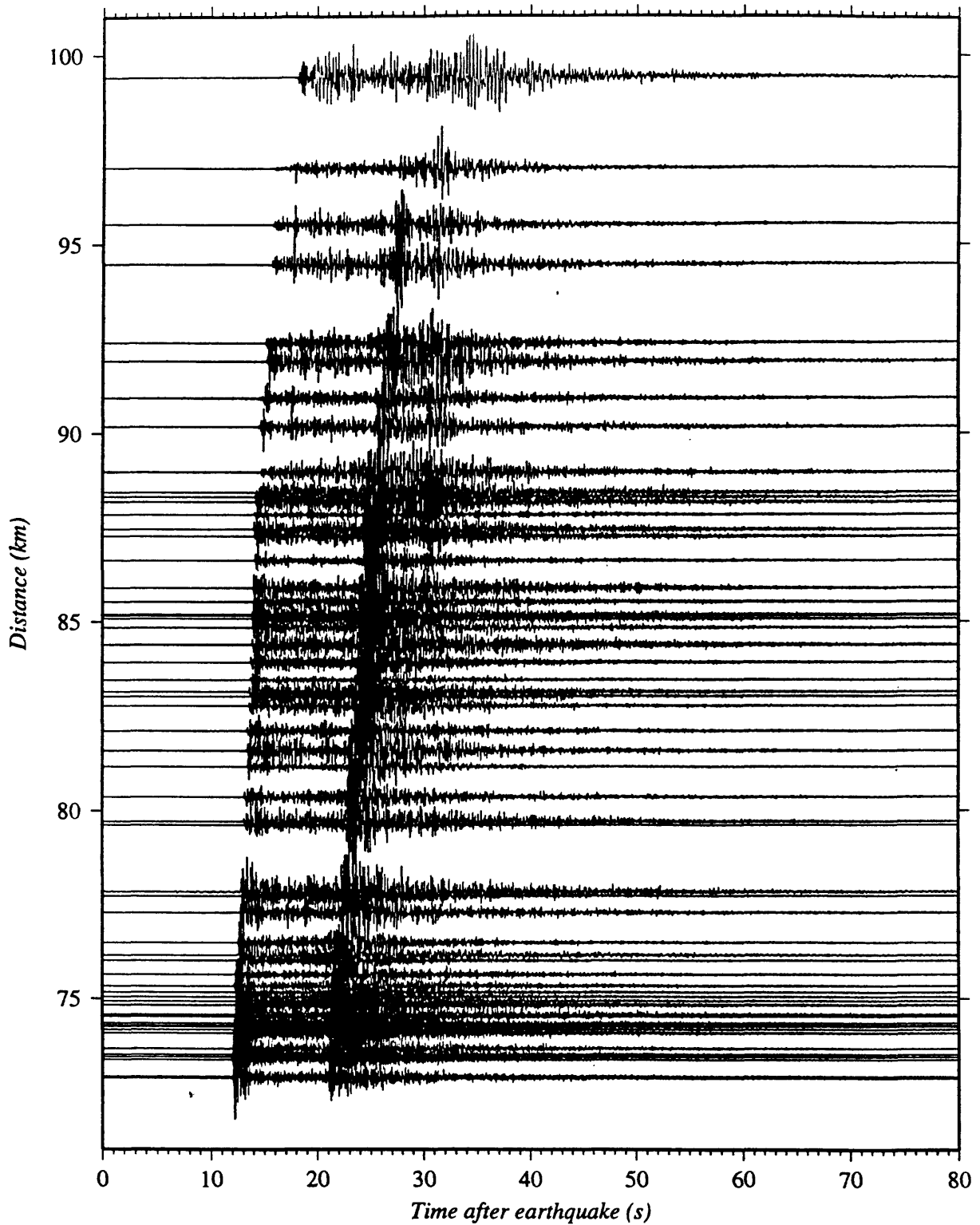
Fig. 7d. Vertical-component record section for local event which occurred on Nov. 28, 1993, 8 km north of Big Bear Lake ( M_L=2.9 ). Travel time (unreduced) after earthquake is shown. See text for details.
