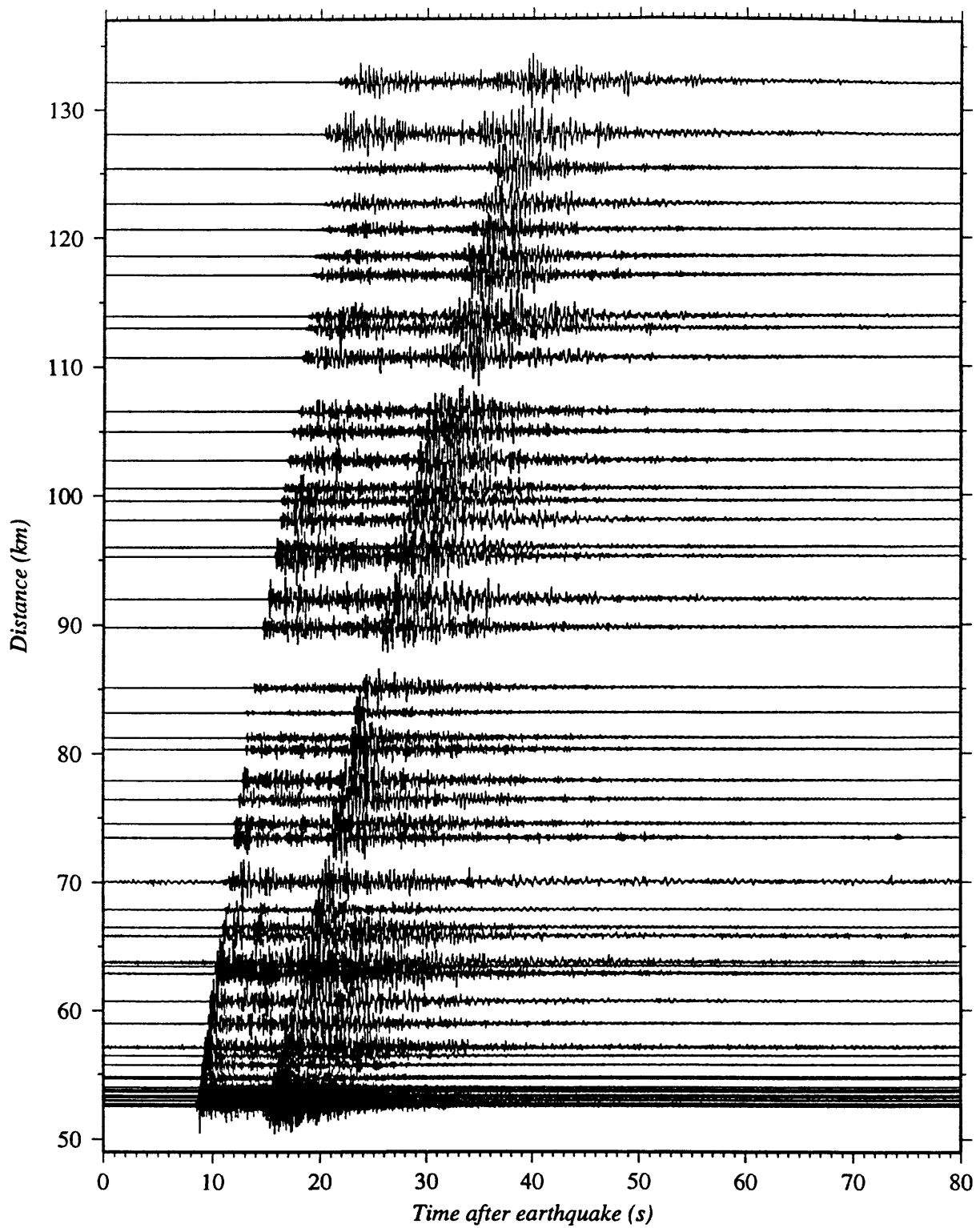
Fig. 7e. Vertical-component record section for local event which occurred on Dec. 3, 1993, 14 km north-northeast of San Fernando ( M_L=2.9 ). Travel time (unreduced) after earthquake is shown. See text for details.
