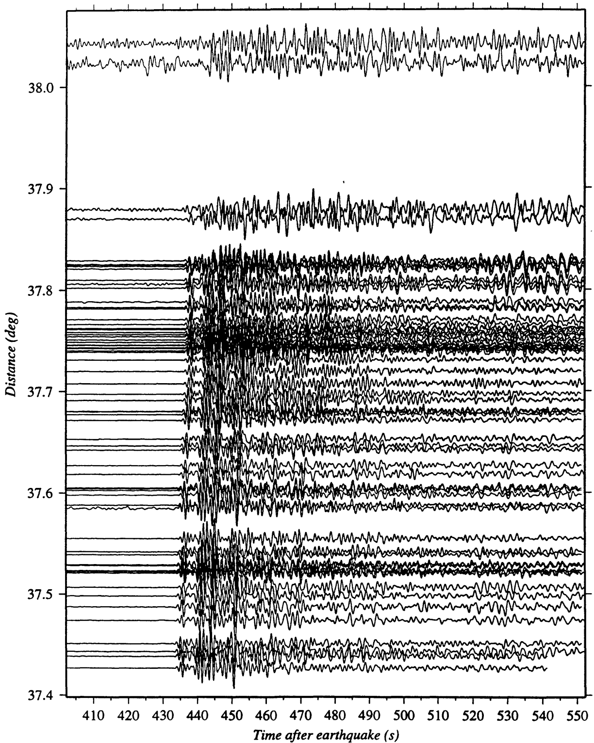
Fig. 6b. Vertical-component record section for teleseismic event which occurred on Nov. 19, 1993 in the Unimak Island Region ( M_w=6.5 ). Travel time (unreduced) after earthquake is shown. See text for details.
