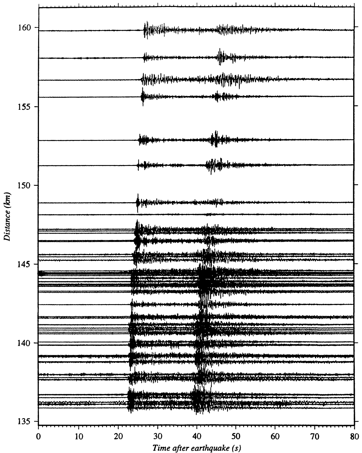
Fig. 7f. Vertical-component record section for local event which occurred on Dec. 4, 1993, 17 km southeast of Yucca Valley ( M_L=2.3 ). Travel time (unreduced) after earthquake is shown. See text for details.
