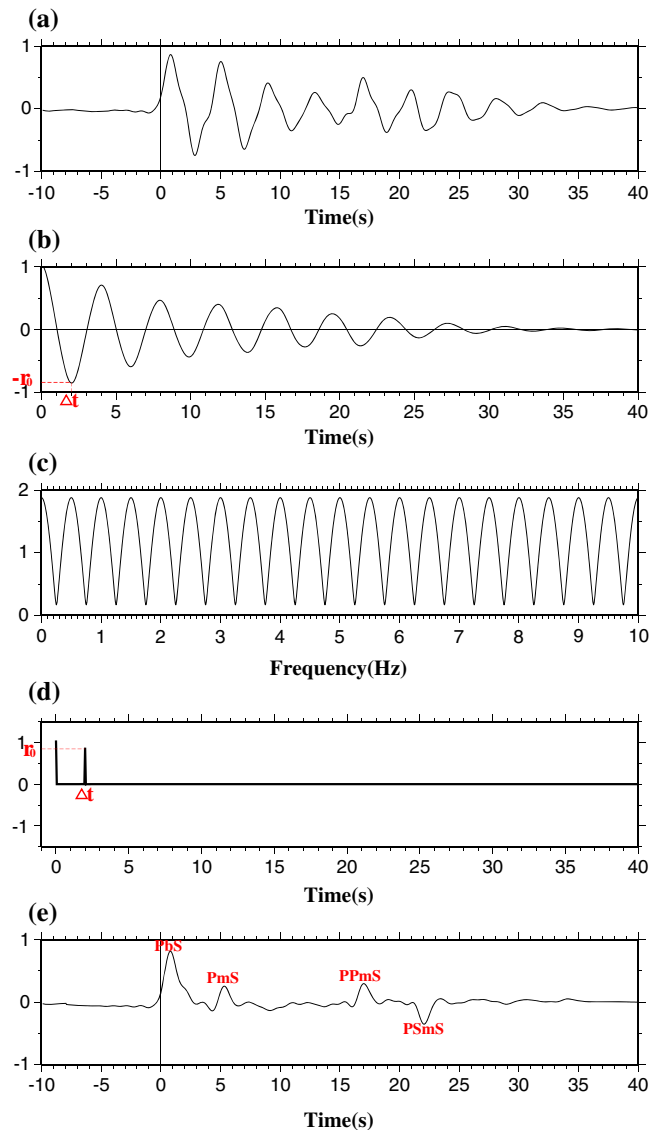
Figure 2. (a) Synthetic RF. Note that the first peak is delayed by about 1 s and represents the P -to- S converted phase from the bottom of the sedimentary layer. (b) Autocorrelation of the RF shown in Figure 2a. \Delta t and r_0 are the two-way traveltime and strength of the sedimentary reverberations, respectively. (c) Frequency domain plot of a resonance removal filter with r_0 = 0.8 and \Delta t = 2.0 s. (d) Same as Figure 2c but in the time domain. (e) Resulting RF after applying the resonance removal filter.
