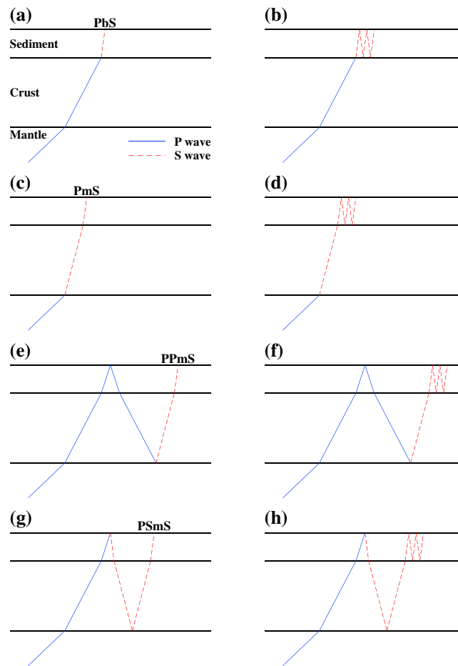
Figure 1. Schematic diagrams showing (a, c, e, and g) the main P_s phases and (b, d, f, and h) their reverberations in the sedimentary layer.
