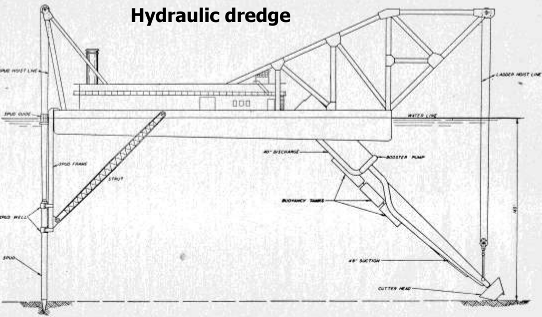
FIG. 100.—PROPOSED 40-IN. HYDRAULIC DREDGE
