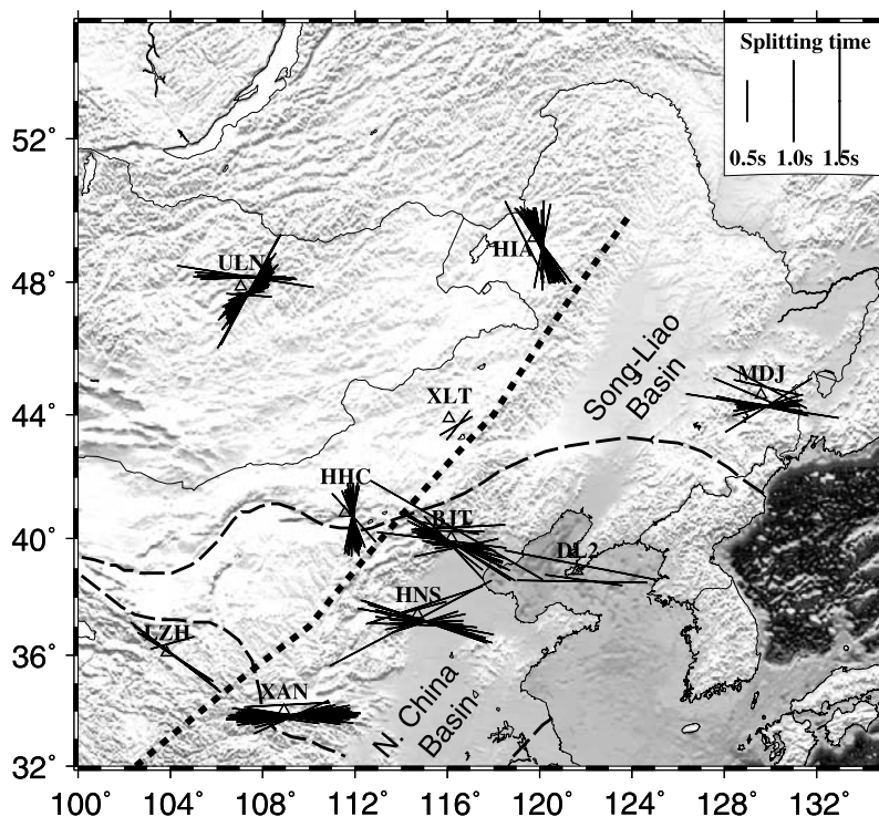
Figure 2. Map showing surface relief and individual SKS splitting measurements in the study area. The orientation of the bars, which are centered at the SKS ray-piercing points at 200 km deep, represents the fast polarization direction, and the length is proportional to the splitting time (see legend at the top right corner for scale). Triangles are stations used in the study. The thick dashed line indicates the boundary between the western and eastern regions of different characteristics of the observed anisotropy. The area between the thin dashed lines is the Archean north China platform, which is bordered by the Qinling-Qilian orogenic belt to the south and the Mongolian arcs terrane to the north [Ren et al. , 1999].
