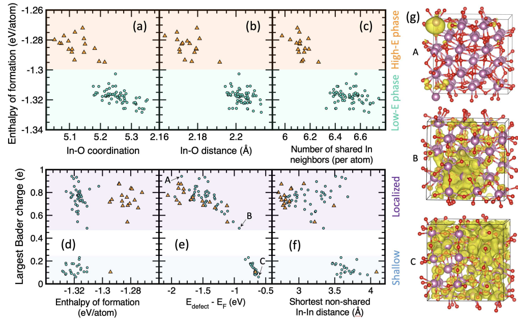
FIG. 2. The structural and electronic properties of 80 a- \text{In}_{54}\text{O}_{79} configurations with different energy and degree of electron localization. (a,b,c) The average In-O effective coordination, the average In-O effective distance, and the average number of shared In neighbors in each of the amorphous structures shown as a function of the corresponding enthalpy of formation. (d) The calculated largest Bader charge in each amorphous configuration for low-energy (circle) and high-energy (triangle) cases. (e) The energy location of the defect state with respect to the Fermi level in each configuration shown for shallow and localized states as determined by the largest Bader charge. (f) The shortest In-In distance for non-shared pairs as a function of the largest Bader charge for each a- \text{In}_{54}\text{O}_{79} . (g) The charge density distribution in the supercell for three representative electronic states—a strongly localized deep trap state (A), a weakly-localized state (B) and a shallow state (C). The three cases are marked in (e).
