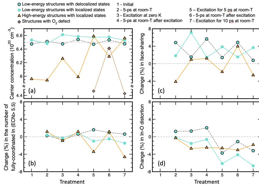
FIG. 3. The calculated carrier concentration and select structural parameters for a\text{-In}_{54}\text{O}_{79} after thermal and/or light treatments marked as 2-7 in the x-axis, see legends and text for more details. The results for 80 structures are presented as an average over the following groups: the low-energy shallow state cases (circle, solid line), the low-energy localized state cases (circle, dash line); the high-energy localized state cases (triangle); and the low- and high-energy structures with \text{O}_2 defect formed (diamond). (a) The number of carriers is given as an average value for the structures in the specified group. (b,c,d) The calculated average percent change with respect to the value in the initial amorphous structure after each treatment. The changes in eight other structural characteristics investigated in this work are at or well below 1%, see SM.
