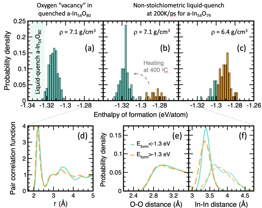
FIG. 1. Distribution of the enthalpy of formation for amorphous \text{In}_{54}\text{O}_{79} structures obtained by different approaches. (a) The results of 880 static-DFT calculations where a single oxygen “vacancy” is created in eleven quenched amorphous \text{In}_{54}\text{O}_{80} configurations by taking out each of the oxygen atoms in the supercell and fully-relaxing the atomic positions at 0 K. The energy distribution for \text{a-In}_{54}\text{O}_{80} are shown by the shared area, whereas the bar plot represents the distribution of 880 calculations for optimized \text{a-In}_{54}\text{O}_{79} . (b) The results of 80 calculations for \text{a-In}_{54}\text{O}_{79} obtained via non-stoichiometric quench simulations that are performed by setting the oxygen stoichiometry at the melting stage of MD, i.e. , prior to cooling. The bi-modal distribution is shown in two colors to mark the difference for the structures with enthalpy of formation above and below -1.3 eV/atom. Heating of the high-energy configurations above 400^\circ\text{C} (via MD simulations with lattice expansion for 5-20 ps) results in lower-energy solutions, see text. (c) The results of 80 non-stoichiometric quench simulations for \text{a-In}_{54}\text{O}_{79} with density 6.4 \text{g/cm}^3 which is 10% below the optimal 7.1 \text{g/cm}^3 used in (a) and (b). The same two-color scheme is used for the single-mode distribution to guide the eye. (d) The average pair correlation function calculated for the low-energy (solid line) and high-energy (dashed line) configurations shown in (b). (e and f) The average O-O and In-In distance distributions calculated for the low-energy (solid line) and high-energy (dashed line) configurations shown in (b). The In-In distribution is further split into edge-shared (thick line) and corner-shared (thin line) In-In pairs.
