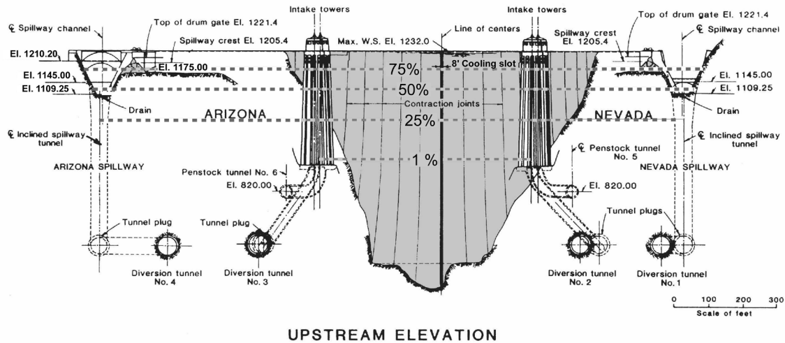
FIG. 4. Upstream elevation view of Hoover Dam, with lines delineating 1%, 25%, 50%, 75%, and 100% levels of the design reservoir storage, based on the original stage curve. The “dead storage” is that zone lying below el. 895, at the base of the intake towers. (USBR)
