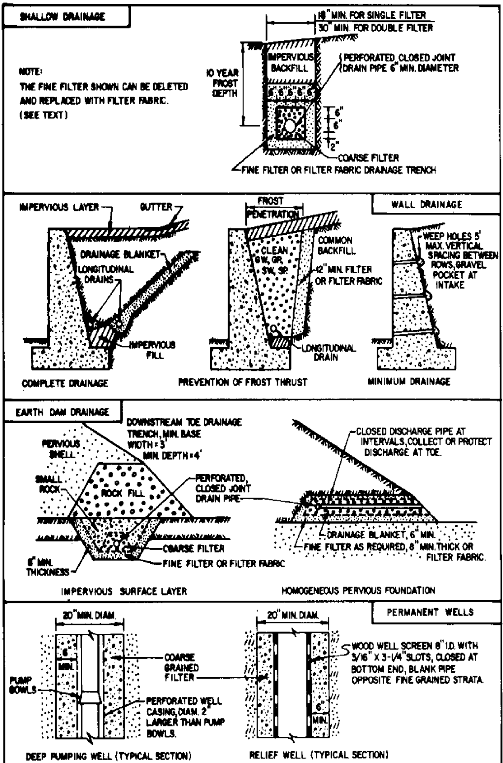
FIGURE 5 Typical Filter and Drainage Blanket Applications
