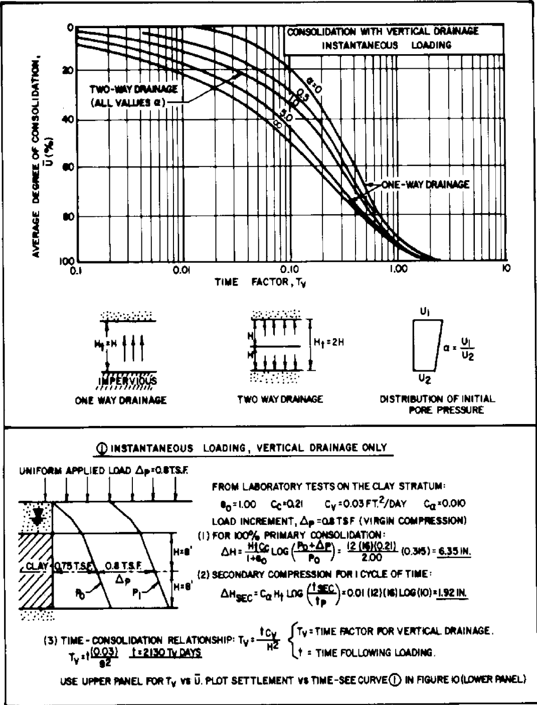
FIGURE 9 Time Rate of Consolidation for Vertical Drainage Due to Instantaneous Loading
