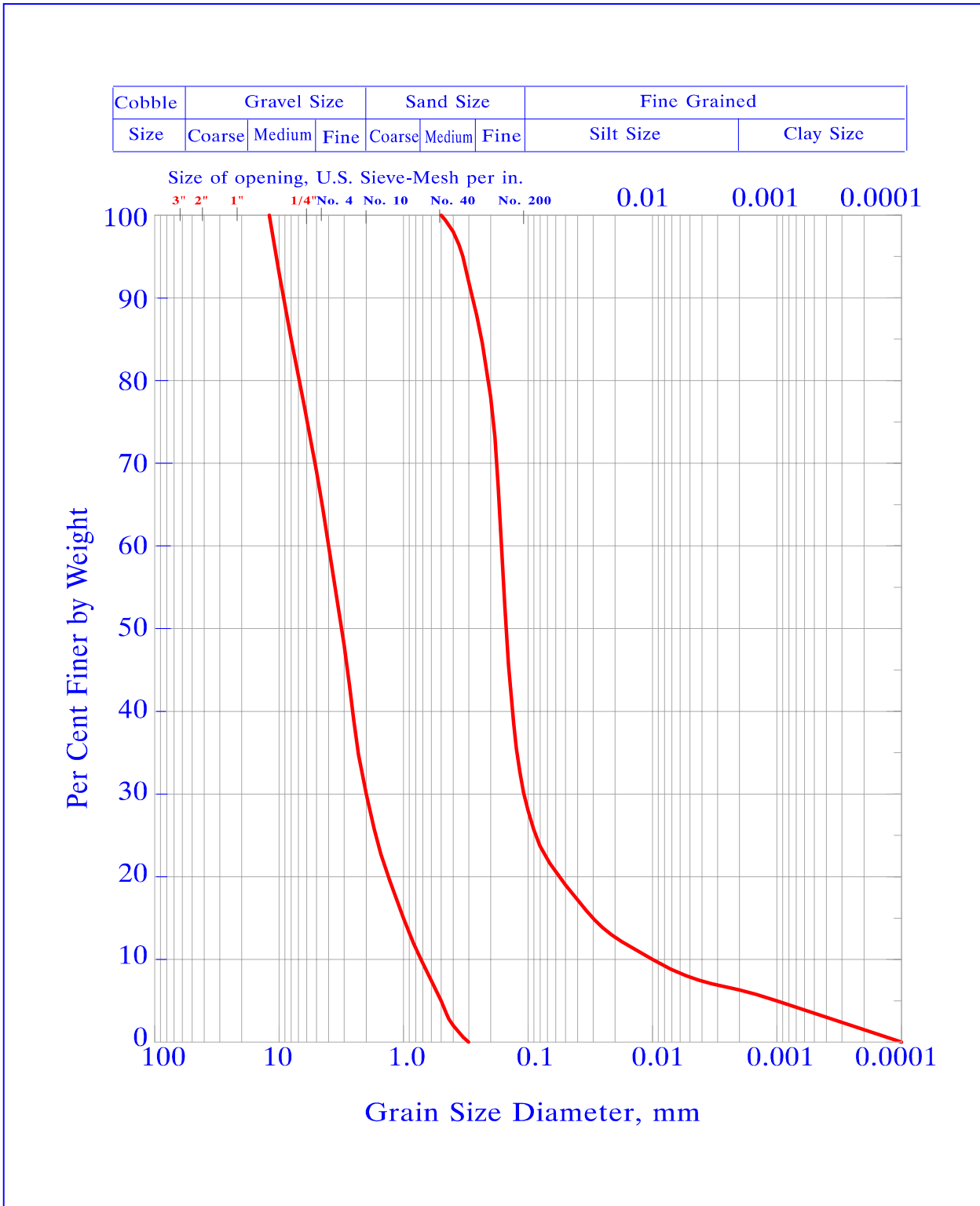
Figure 12 Grain Size Ranges Considered for Vibro-Densification
