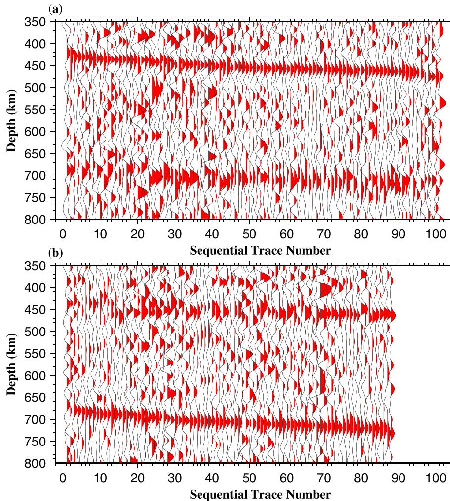
Figure 3. (a) Results of stacking all available normal moveout corrected RFs from 1^\circ radius bins with a minimum of 10 high-quality RFs, plotted with sequentially increasing depth of the d410 . (b) Same as (a) but for sequentially increasing depth of the d660 .
