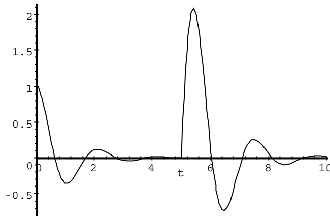
Figure 3. System response to time-shifted impulse
