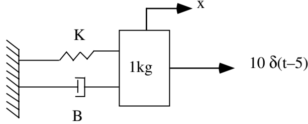
Figure 1. Impulsively forced spring-mass-damper system – use Laplace transformation
