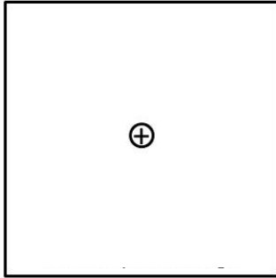
Positive point charge
