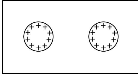
Two insulating spheres coated with positive surface charge
