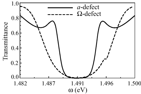
Fig. 1. Numerically generated transmission spectra of GaInAs/GaAs MQW's with \Omega - (dashed line) and a - (solid line) defects. Input parameters were chosen from Ref. [3]: \Omega_0 = 1.491 eV, \Gamma_0 = 27 \mu eV, and exciton relaxation parameter \gamma_{hom} = 0.28 meV. The length of the system is N = 200 .
