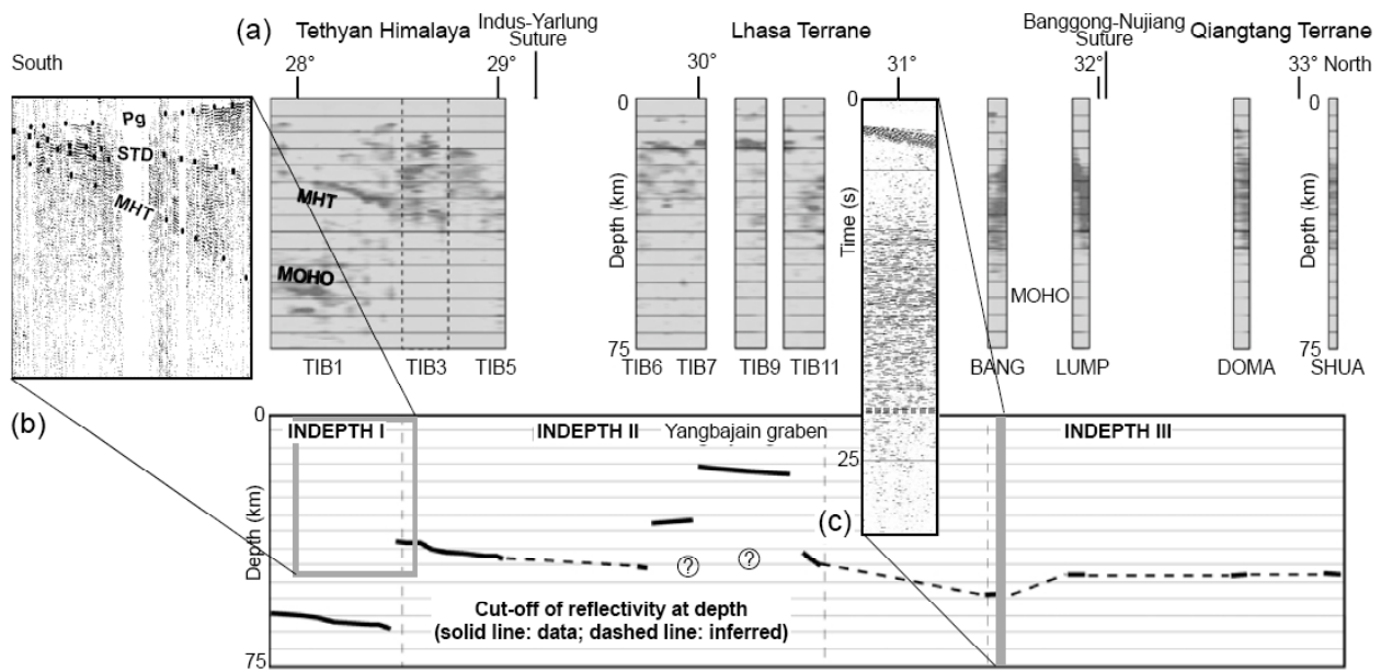
Figure 6. Vertical distribution of crustal reflectivity from INDEPTH profiling along \sim 90^\circ\text{E} . (a) Reflection strength along INDEPTH stacked vertical reflection profiles (above) and interpreted cut-off of reflectivity at depth (below). From the south: on profile TIB-1 (IN-1), clear Moho and Main Himalayan Thrust (MHT) reflections are seen; on TIB-1, -3 and -5 (IN-2) reflectivity is strongest above the MHT; TIB-6, -7, -9, and -11 (IN-2) are dominated by reflectivity around 15 km depth (seismic bright-spots) but question marks indicate uncertainty as to whether high attenuation is preventing observation of reflective layering at depth; from the middle of TIB-11 north, including profiles BANG, LUMP, DOMA and SHUA (IN-3), mid-crustal reflectivity is replaced by lower-crustal reflectivity that terminates at the Moho. Vertical exaggeration is \times 2 . After Ross et al. (2004). (b) Inset of wide-angle reflection data (time-domain receiver gather with reduction velocity of 6 \text{ km}\cdot\text{s}^{-1} ) at south end of profile; approximate extent shown by grey box on reflectivity cut-off plot, showing prominent reflectivity between STD and MHT. Pg is direct wave. Note that upward convergence of STD and MHT to the south is an artifact of the receiver-gather display in which true geometries are highly distorted; these reflectors are actually sub-parallel. After Makovsky et al. (1996). (c) Inset of near-vertical reflection data (time-domain shot gather with no move-out) from BANG profile, at same vertical (travel-time) scale as inset (b) but very different horizontal (distance) scale, to show absence of upper-crustal reflectivity and clear middle-to-lower-crustal reflectivity; amplitude-decay curves show shot-energy extends below Moho (interpreted at 22 s travel-time (63 km), grey dotted line) so reflectivity cut-off has tectonic significance. After Ross et al. (2004).
