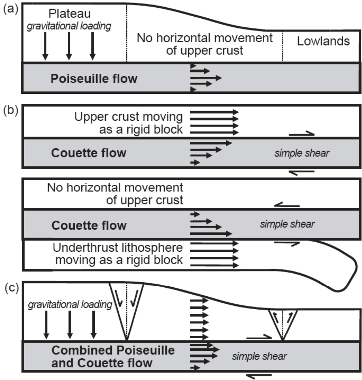
Figure 2. Modes of channel flow with imposed rigid boundary conditions.
