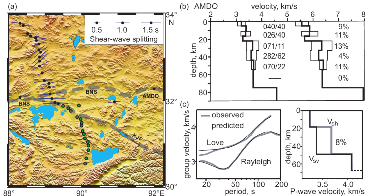
Figure 5. Evidence for crustal seismic anisotropy.
