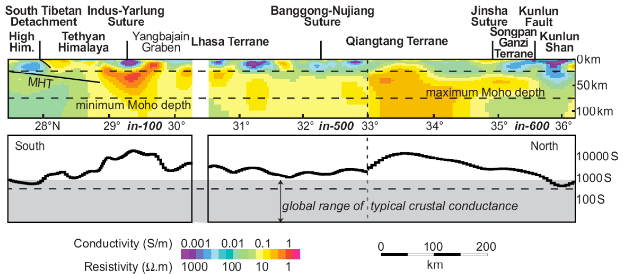
Figure 4. Lithospheric electrical conductivity of Tibetan Plateau, modified after Wei et al. (2001).
