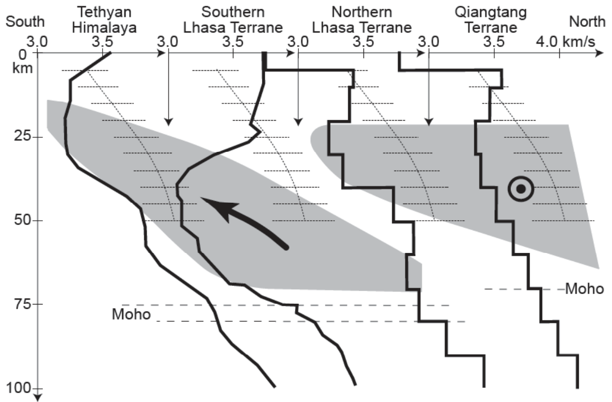
Figure 3. Surface-wave velocity models along IN-1, -2 and -3.
