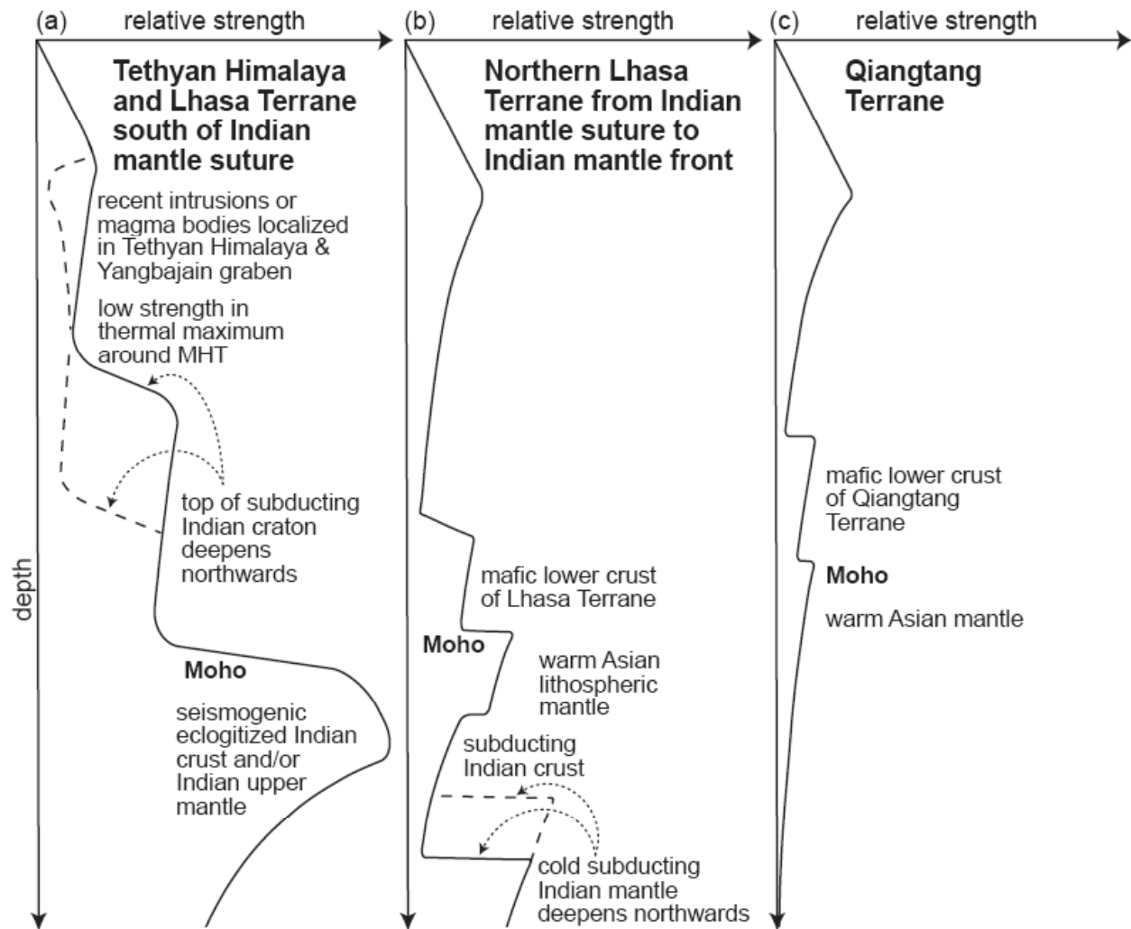
Figure 7. Cartoons of inferred relative strength-depth profiles for Tibet at about 90°E.
