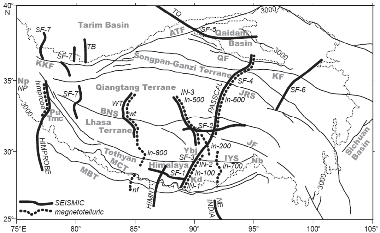
Figure 1. Location map of main geophysical experiments referred to in this paper.
