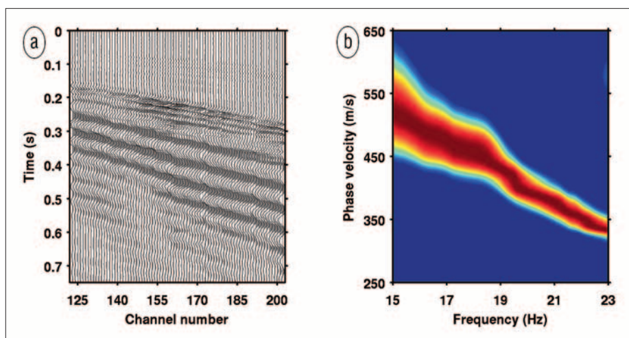
Figure 13. Section of a trace-normalized DAS shot gather for the inline source (a) and associated normalized dispersion spectrum (b) calculated in the frequency slowness domain. As can be seen in (a), while the refracted P-wave arrival is weak, a direct S-wave and a strong Rayleigh-wave package are visible. The dispersion plot in (b) shows the fundamental mode is normally dispersive from 15 to 23 Hz.
