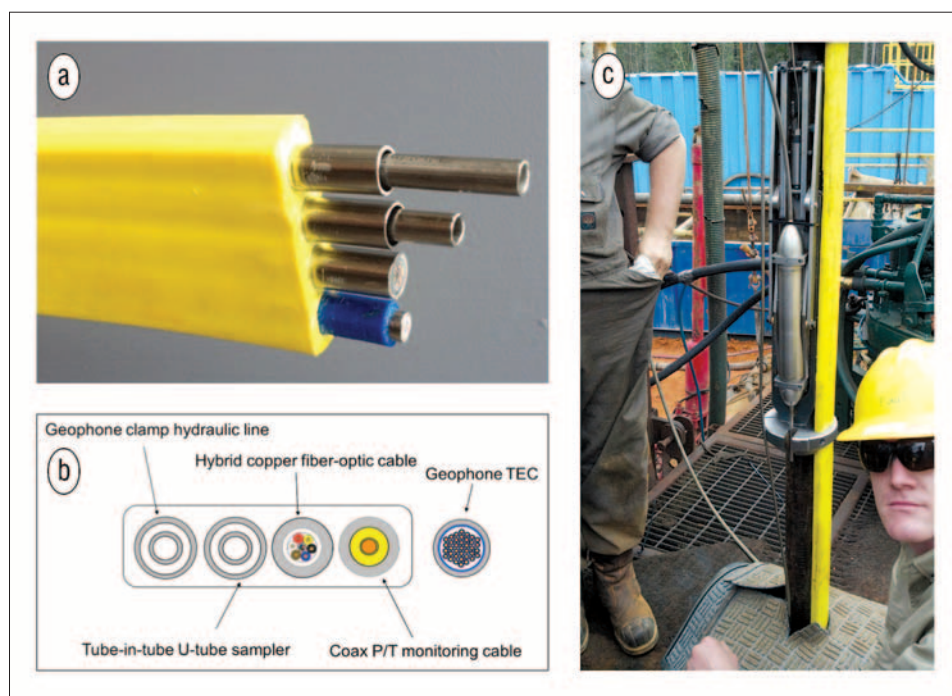
Figure 1. Flatpack with DAS cable photo (a) and schematic (b). Note that the geophone tubing encapsulated conductor (TEC) cable was deployed separately from the flatpack. (c) Flatpack and wall-locking geophone clamped on tubing.
