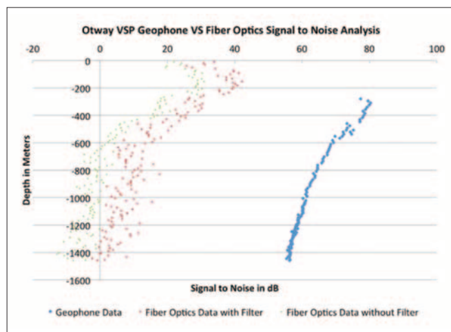
Figure 8. Comparison of P-wave signal-to-noise ratio (SNR) for wireline, clamped geophones and tubing-deployed DAS fiber-optic from separate VSP surveys in the same well. Filtered fiber data has a band-pass filter of 5–180 Hz applied to improve SNR. Different sources were used in the two data sets. To obtain SNR, the root-mean-squared (rms) amplitude values for a 20-ms time window around the P-wave arrival is compared to early time pre-arrival noise.
