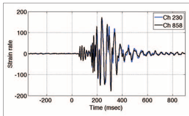
Figure 10. Comparison of two 1-m segments of cable collocated in a surface trench.
