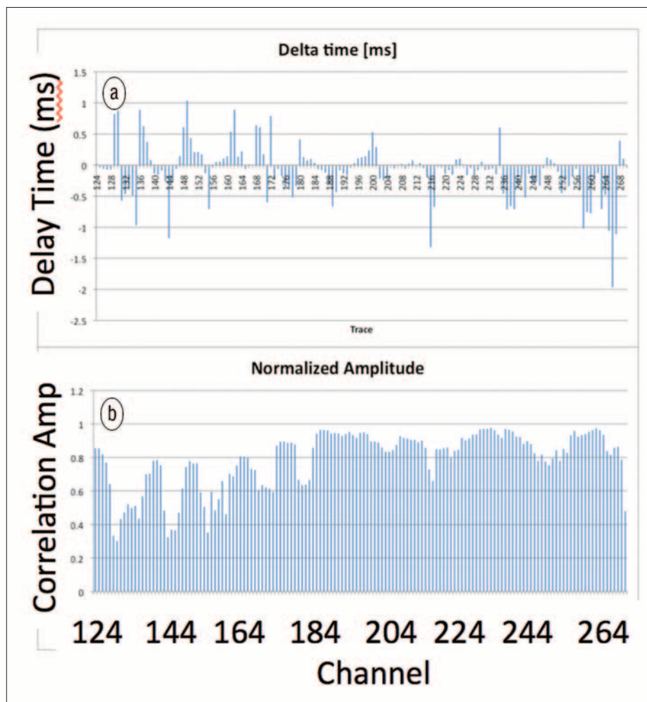
Figure 11. Cross-correlation results for two sections of surface cable colocated in trench showing, for each meter of cable (trace #), the relative time delay (a) and the normalized cross-correlation coefficient (b).
