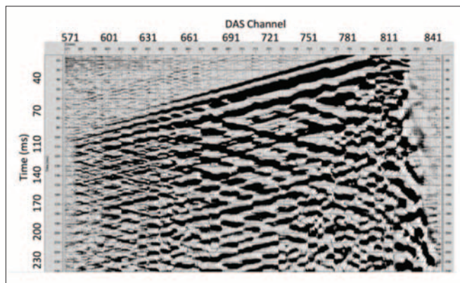
Figure 14. Raw DAS VSP data from upper 300 m in the Ketzin Ktzi 202 borehole for a stack of 92 source drops. DAS channels have 1-m spacing and the fiber cable is installed behind casing. The downgoing P-wave and upgoing reflections can be seen.
