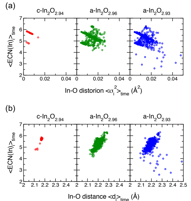
FIG. 10. The time-average effective coordination number (ECN) for every In atom in the cell for crystalline and amorphous non-stoichiometric \text{In}_2\text{O}_x (a) as a function of the average distortion; and (b) a function of time-average In-O distance. Every data point represents a time average over 3,000 MD configurations (6 ps) obtained at 300 K. For amorphous cases, the results of 10 separate MD realizations in each case are shown.
