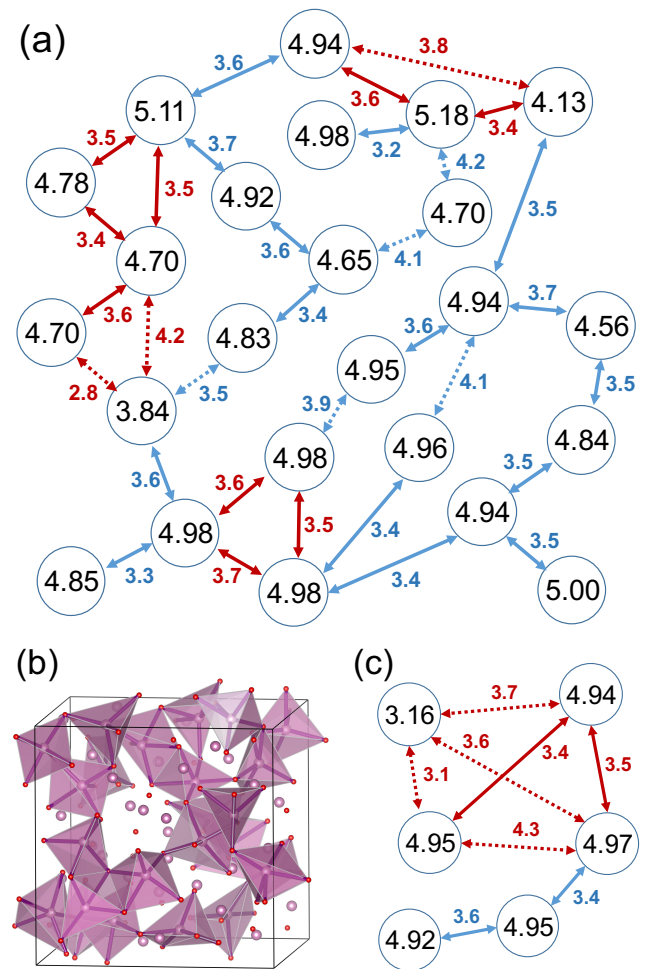
FIG. 15. (a) Schematic representation of the under-coordinated under-shared In atoms in one of the a\text{-In}_2\text{O}_{2.93} structures with the largest fraction of such In pairs. Solid lines represent corner-shared connections, while dashed lines represent non-shared connections between pairs of In atoms. The In-In distances (in Å) are given next to each connection. Loops of 3 atoms are highlighted with red. (b) The same under-coordinated under-shared In atoms as shown in (a) are shown here as highlighted polyhedra in the supercell of a\text{-In}_2\text{O}_{2.93} . (c) Schematic representation of the under-coordinated under-shared In atoms in one of the a\text{-In}_2\text{O}_{2.93} structures with 4-atom loop that represents the biggest cluster of under-shared under-coordinated In atoms.
