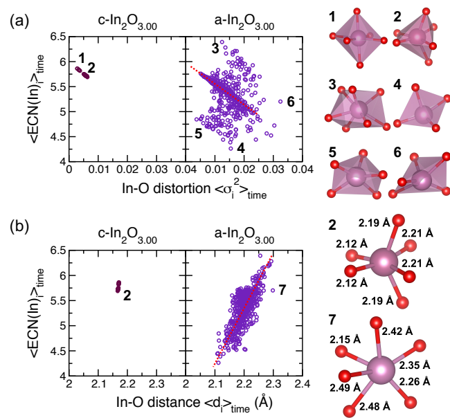
FIG. 4. The average effective coordination number (ECN) for individual In atoms in the cell for crystalline and amorphous stoichiometric \text{In}_2\text{O}_3 (a) as a function of the time-average distortion of the In atom; and (b) a function of time-average In-O distance of the In atom. Every data point represents a time average over 3,000 MD configurations (6 ps) obtained at 300 K. For amorphous case, the results of 10 separate MD realizations are shown. The dotted red lines are to guide the eyes. Representative In-O polyhedra for both crystalline and amorphous \text{In}_2\text{O}_3 are shown on the right to highlight severe distortions or longer-than-average distances in the specific polyhedra.
