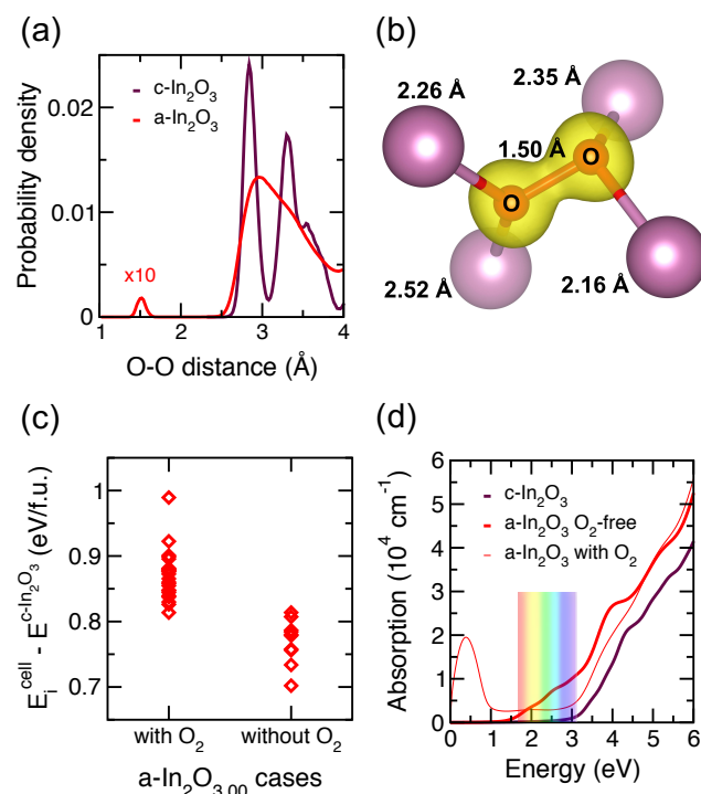
FIG. 9. (a) Calculated O-O distance distribution in stoichiometric crystalline and amorphous \text{In}_2\text{O}_3 , as obtained from the 3,000 MD simulations at 300 K. For a- \text{In}_2\text{O}_3 , the plot represents 25 MD realizations. (b) Charge density distribution isosurface for \text{O}_2 defect in stoichiometric a- \text{In}_2\text{O}_3 and the distances from each to their nearest In neighbors. (c) Total energy of 35 amorphous stoichiometric \text{In}_2\text{O}_3 cells calculated with respect to the total energy of crystalline stoichiometric \text{In}_2\text{O}_3 . A few states with \text{O}_2 have a total energy lower than states without \text{O}_2 , indicating possible spontaneous formation of \text{O}_2 defects in rapidly quenched \text{In}_2\text{O}_3 . All values are obtained using hybrid functional (HSE06) calculations for the structures optimized using DFT-PBE. (d) Calculated optical absorption in stoichiometric crystalline and amorphous \text{In}_2\text{O}_3 obtained using hybrid functional (HSE06) calculations for the structures optimized using DFT-PBE. For the amorphous oxide, the average over 10 MD+DFT(HSE) realizations (with no \text{O}_2 ) and over 25 MD+DFT(HSE) realizations (with \text{O}_2 formed) are shown.
