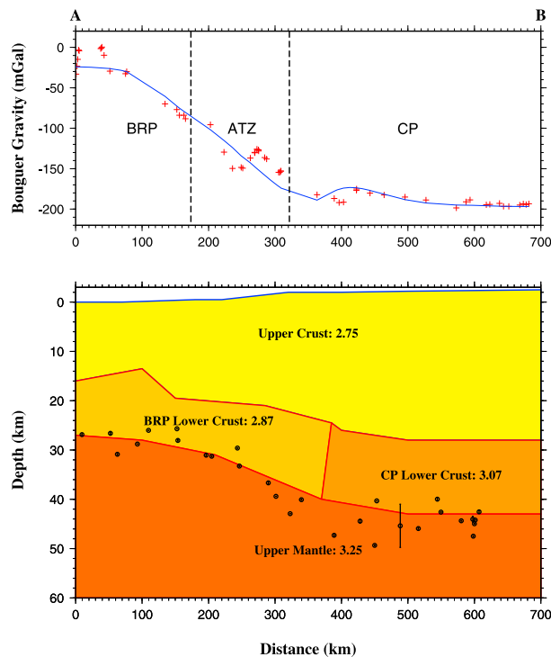
Figure 9. Gravity model of the crust and upper mantle along profile A-B (Figure 5). Densities are in \text{g/cm}^3 . The red crosses are observed and the blue line is calculated gravity anomalies. Dots represent crustal thickness determinations at stations in the 200 km wide band centered on the profile.
